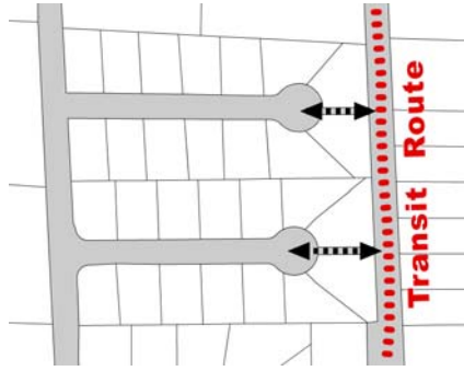
Figure 8a - Preferred; direct pedestrian access to transit
