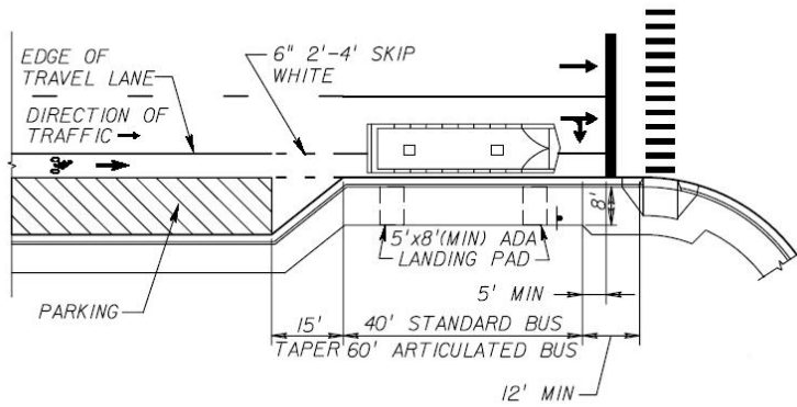
Figure 20 - Near-Side Bus Bulb
