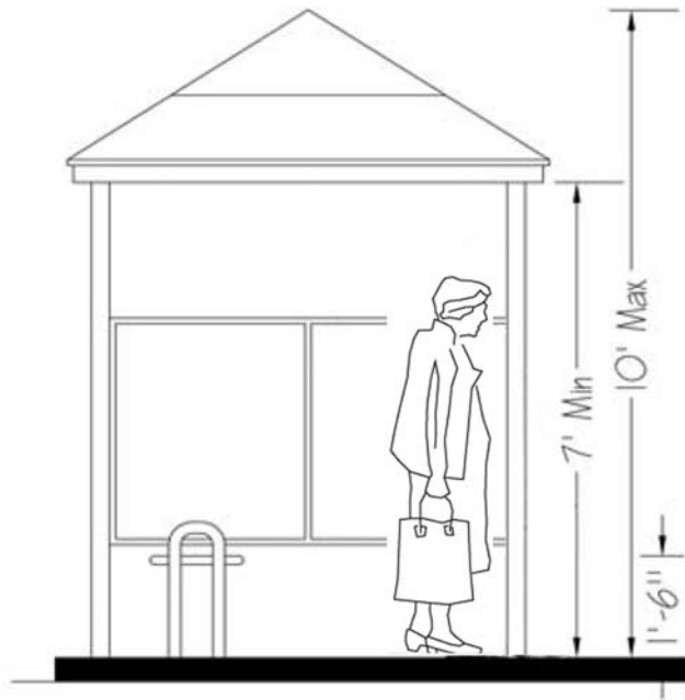
Figure 27 - Cross section of a mid-size shelter with typical vertical dimensions.
