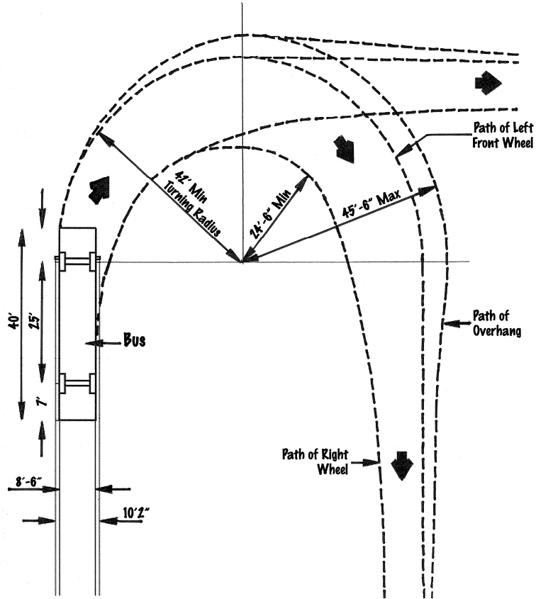
Figure 13 - Standard Bus Turning Template
