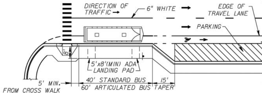
Figure 22 - Far Side Bus Bulb
