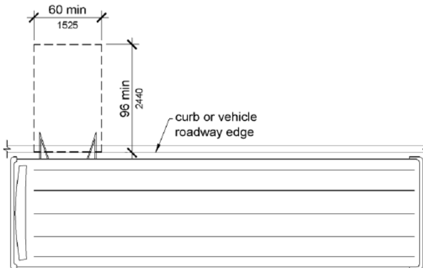
Figure 29 - Dimensions of Bus Boarding and Alighting Areas
